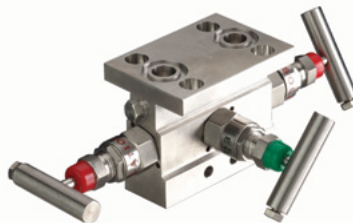
3 VALVE; "T" Style; Remote Mount; 316/L; 1/2" NPT (F) x FLG x 1/4" NPT Drain/Vent; 6000 psi; PTFE Packing
