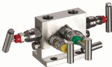
5 VALVE; "T" Style; Remote Mount; 316/L; 1/2" NPT (F) x FLG x 1/4" NPT Drain/Vent; 6000 psi; PTFE Packing
