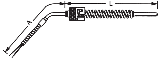
MODEL PTSA (Locking nut travels on coiled spring)
