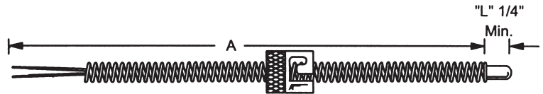
MODEL PTAF (Locking nut travels on flex armour)
